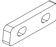
Rear Mounting Bracket Spacer Part # 200415823 Qty 2
